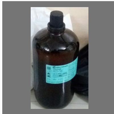
Acetone Chemical
